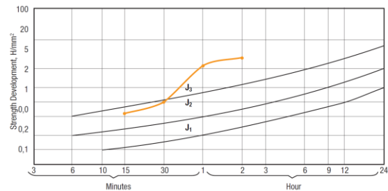
Early Strength Development
